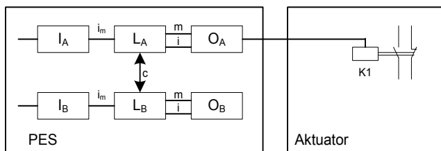
Single-channel output PSC1 and single-channel actuator without diagnostics
