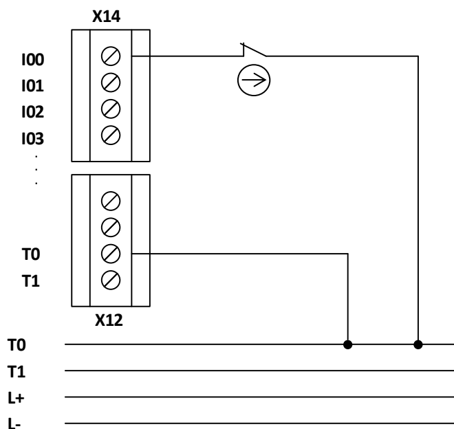
Single-channel sensor with test pulses
