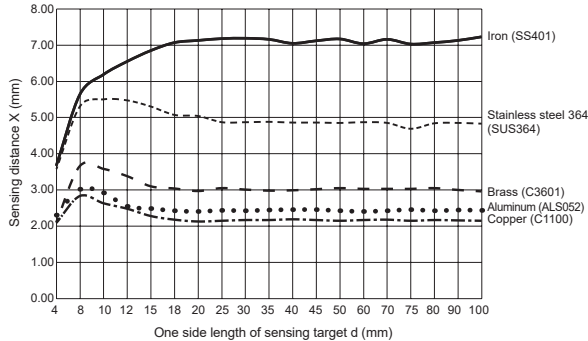
● PRD(L)T30-15D
