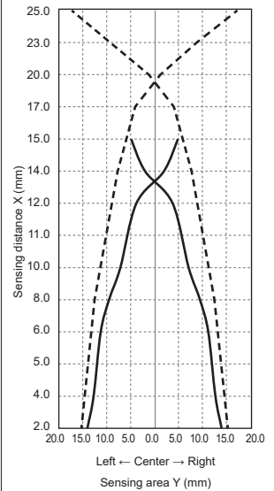
● PRD(L)T30-15D□/25D□
