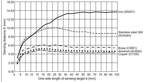
● PRD(L)T30-25D
