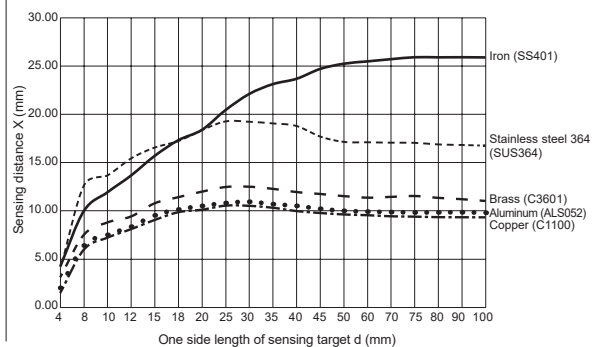
● PRD(L)T30-25D
