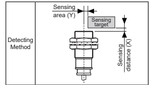
● PRD(L)T30-15D□/25D□
